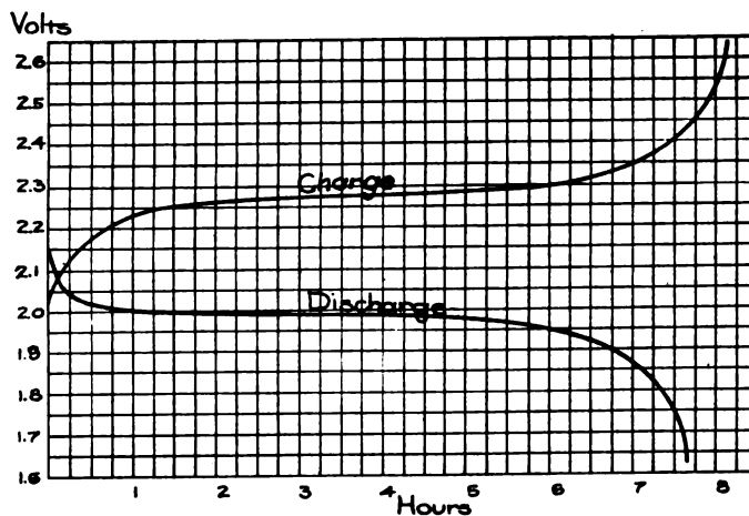
Typical Diagram of Charge and Discharge.
